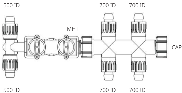
5 RVTT5-MHT + RSI47 (Pre Assembled)
